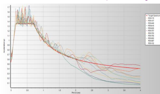
Fig. 4. Scaled Spectrum of earthquake records on soil Type III according to Standard No. 2800
