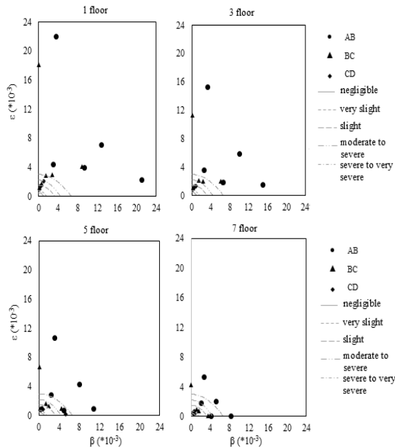
Fig. 20. Diagrams of singular footing damage, at different loading and for different positions of the pipe after one month
