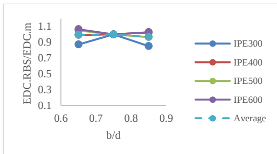
Fig. 26. Variation of EDC.RBS/EDC.m with respect to b/d
