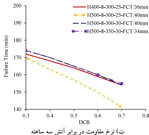
Fig. 5. Column failure time versus DCR
