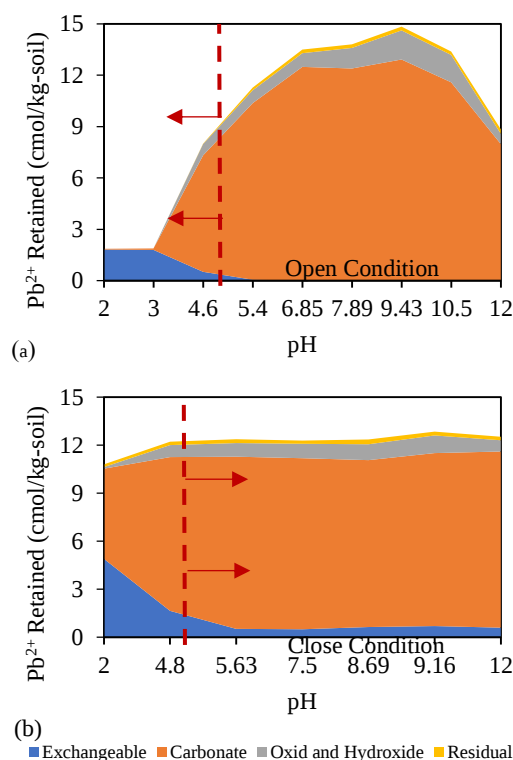
Fig. 3. Variations of retained \text{Pb}^{2+} by different phases of kaolinite at various pH for kaolinite with 15 cmol/kg-soil \text{Pb}(\text{NO}_3)_2 - (a): Open Condition, (b): Close Condition
