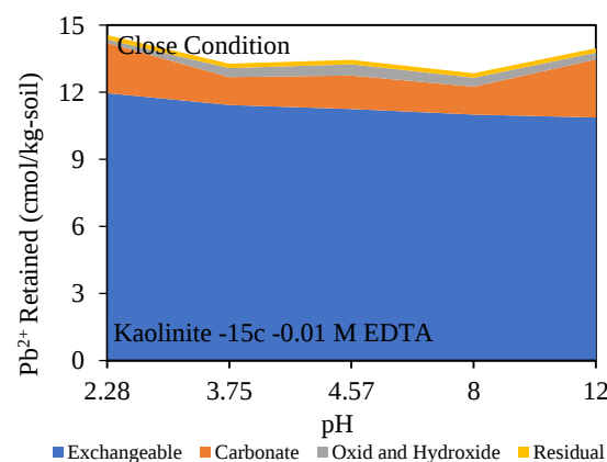
Fig. 6. Variations of Pb^{2+} retained by different phases at various pH for kaolinite with 15 cmol/kg-soil Pb(NO_3)_2 and enhanced by 0.01 Molar EDTA
