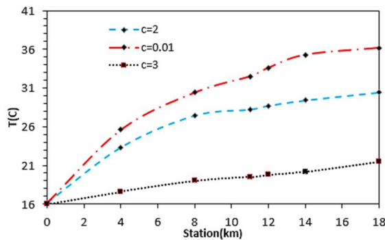
Fig. 6. Sensitivity analysis for the water temperature- "c" parameter-April 2013
