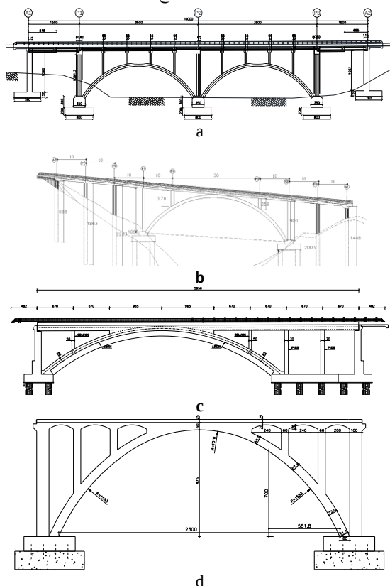
Fig. 2. General layout of the studied bridges: a) Siah-Bisheh; b) Gazanak; c) Vana; and d) Ziabagh.
