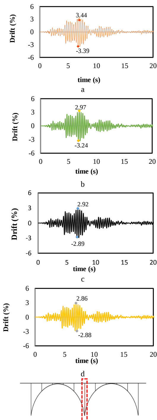
Fig 5. Drift history of the middle column of the Siahbisheh bridge with the applied angles of: a)90; b)60; c)30; and d) 0 degrees under the Kobe earthquake.
