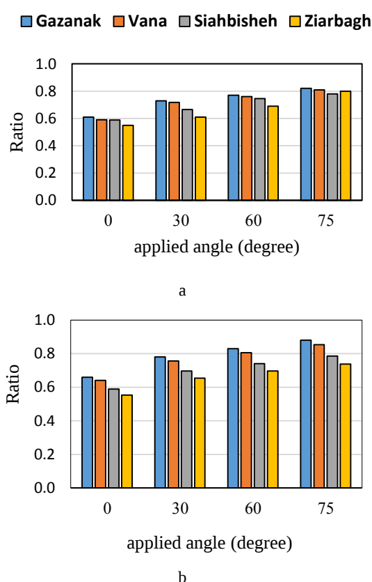
Fig. 6. (a) Ratio of curvature at arch midspan under different angles to the corresponding value with the 90-degree incidence angle under the Manjil earthquake; (b) Ratio of curvature ductility demand at arch midspan under different incidence angles to the value corresponding to the 90-degree angle under the Kocaeli earthquake
