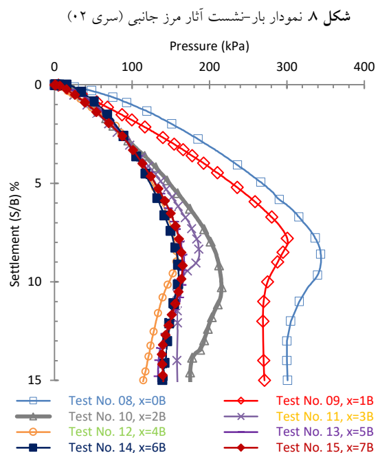
Fig. 8. Pressure-settlement curves with different x/B ratios
