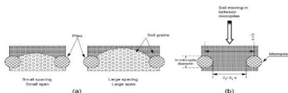
Fig. 14. (a) Mechanism of confinement with confining piles (Unnikrishnan, N., & Sachin, 2009), (b) plastically deforming soil between two adjacent micropiles
