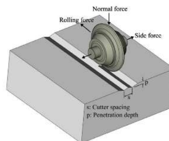
Fig. 1. Rock cutting forces [1]
