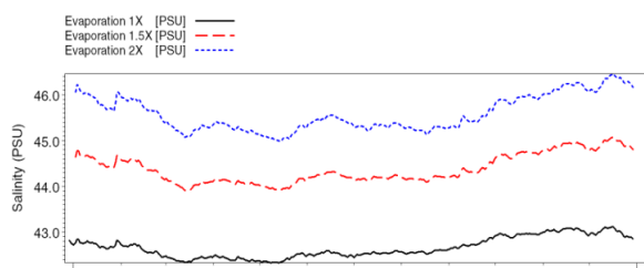
Fig. 13. The average salinity of the surface of the Persian Gulf with the change of evaporation rate
