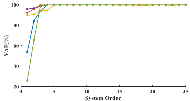
Fig. 7. Variance Account for (VAF) of damaged building with RMS (0%, 7%).
