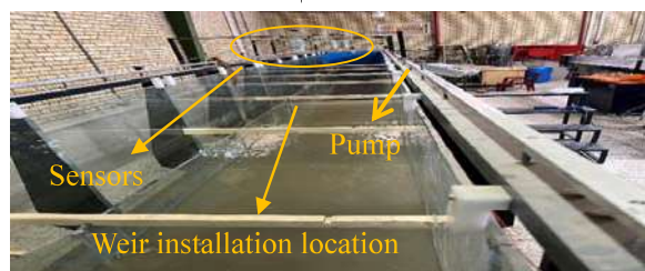
Fig. 2. A view of the experimental flume
