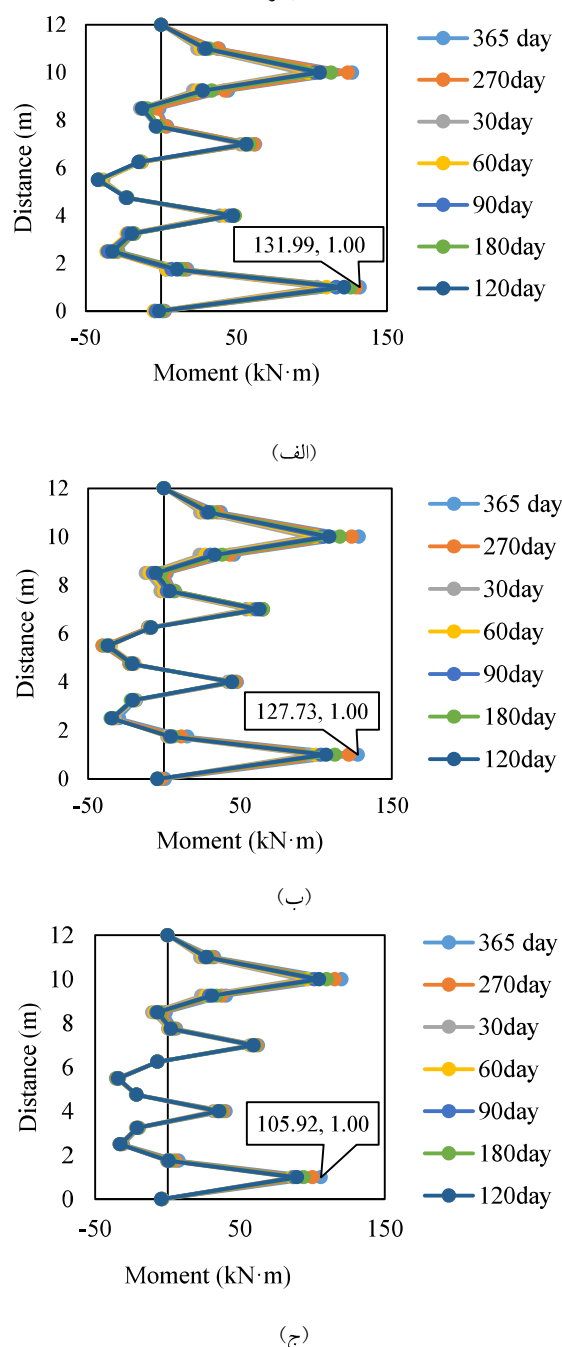
Fig. ۵ Diagram of bending moment-depth of the excavation wall for the stabilization excavation by anchoring method in the vicinity of the absorption well. a) 3 meters, b) 5 meters, c) 8 meters from Jadhargod
