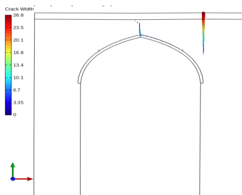
Fig. 14. The distribution pattern of cracks at the ultimate shear capacity for the wall with 0.1 MPa pre-compression gravity load intensity (average displacement of 25.9 mm at the top of the wall)
