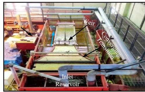
Fig. 3. Experimental flume
