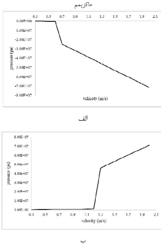
Fig. 8. Changes of pressure in relation to speed a) minimum pressure, b) maximum pressure
