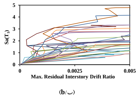
Fig. 5. IDA curves of the 4-story RBRBF structure corresponding to the MRIDR = 0.5% under: (a) subduction and (b) crustal records
