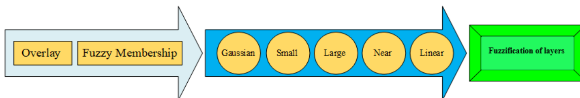
Fig.3. Fuzzy diagram of Euclidean distance maps with Fuzzy operators in ArcGIS
