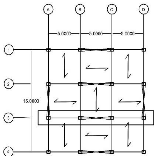
Fig. 1. The position of frames in the plan and the schematic view of brace arrangement
