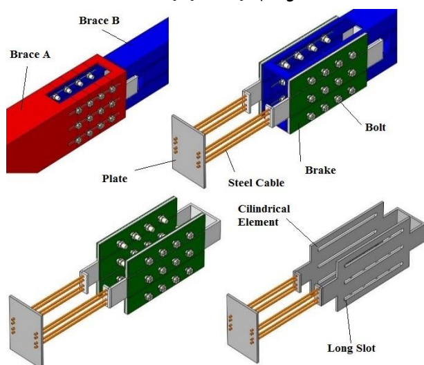
Fig. 3. FCFD damper configuration
