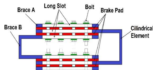
Fig. 5. Non-slip FCFD damper plates
