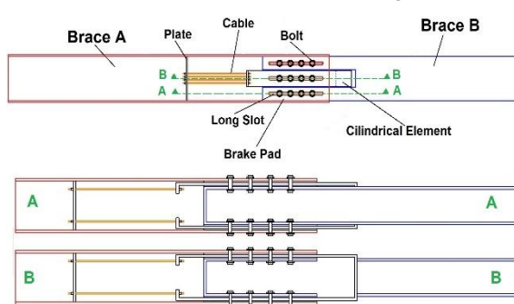
Fig. 4. FCFD Damper Modeling
