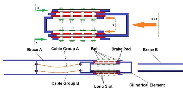
Fig. 6. Slippage of FCFD damper plates in pressure
