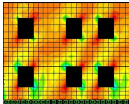
Fig. 5. Contour of the maximum principal stress in a typical external wall of case#1 with RC ties
