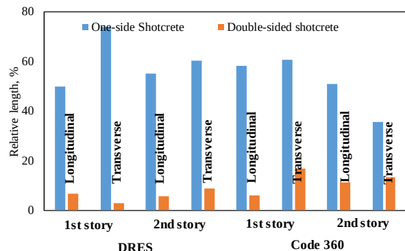
Fig. 6. Average of the retrofitted walls relative length (Flexible diaphragm w/o ties)
