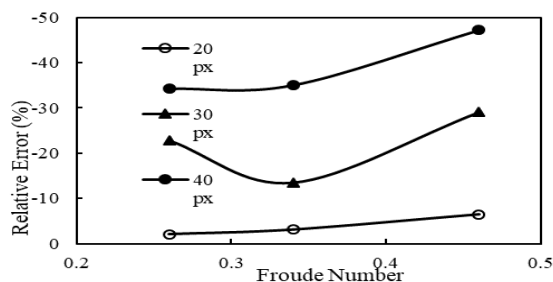
Fig. 8. The relative error of flow rate measurement in the laboratory channel in terms of Froude number for different dimensions of the exploration window
