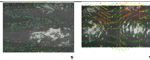
Fig. 5. Examining the effect of camera positioning (1) installation in the center of the channel vertically (2) installation at the entrance of the channel obliquely; Average flow surface velocity vectors in the laboratory channel at a depth of 15.5 cm for two positions of the camera inclined mode (3), vertical mode (4)
