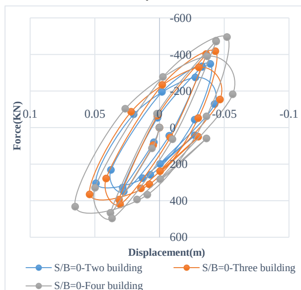
Fig. 13. Investigating the effect of the number of structures on hysteresis diagram of the liquefaction soil layer
