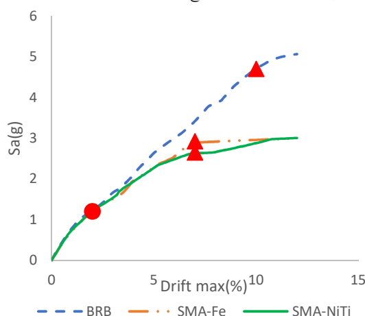
Fig. 16. Comparison of average level IDA curves for all three different braces
