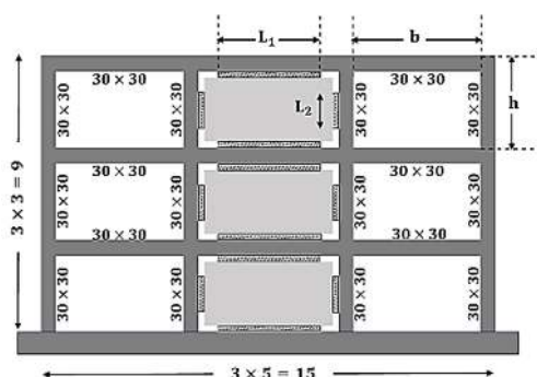
Fig. 2. Modeled frame specifications
