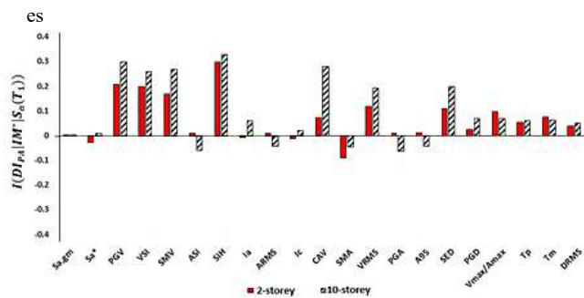
Fig. 10. Comparison of relative entropy of different intensity measures for two- and ten-story fram
