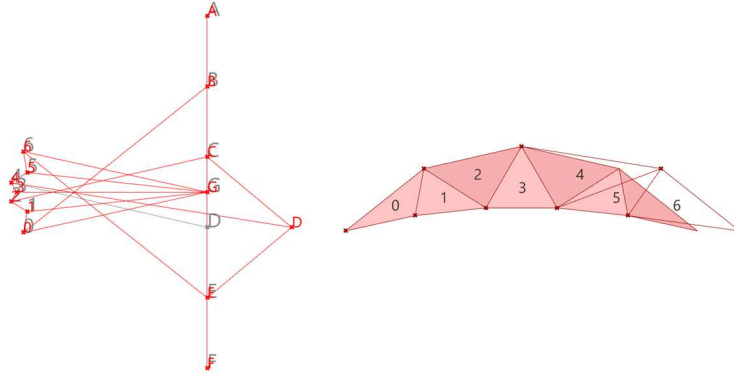
Fig. 9. Changes made in the force diagram and redraw the form diagram corresponding to the changes
