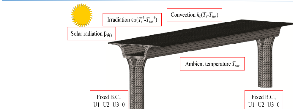
Fig. 7. Finite element model of the bridge constructed with ABAQUS Software
