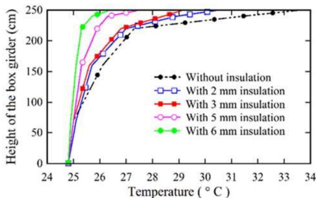
Fig. 16. Vertical temperature gradient with and without insulations at 1430 hrs
