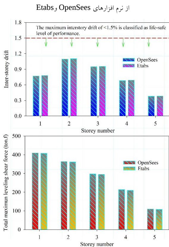
Fig. 5. Comparison of drift and total maximum levelling shear force of 5-storey structure from OpenSees and Etabs softwares
