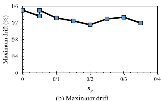
Fig. 11. Effect of increasing prestressing force ratio on drift
