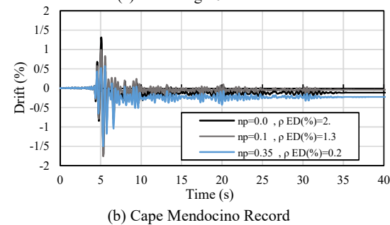
Fig. 10. Comparison between drift histories with different prestressing force ratios
