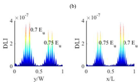
Fig. 9. 1 st mode DLI diagram of the D3 damage state with the damage severity (a) 10%, (b) 20% and (c) 30%
