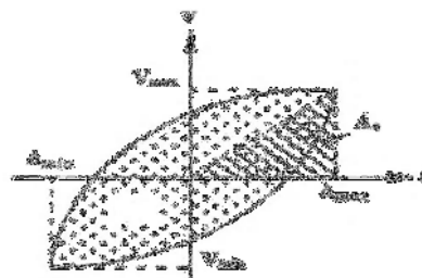
Figure 20. The force-displacement curve for equivalent hysteresis damping [29]
