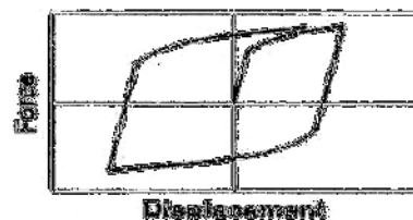
Figure 21. Idealized hysteresis behavior of Hysteretic damper [30]
