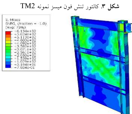
Fig. 3. Von Mises stress contour of TM2 specimen
