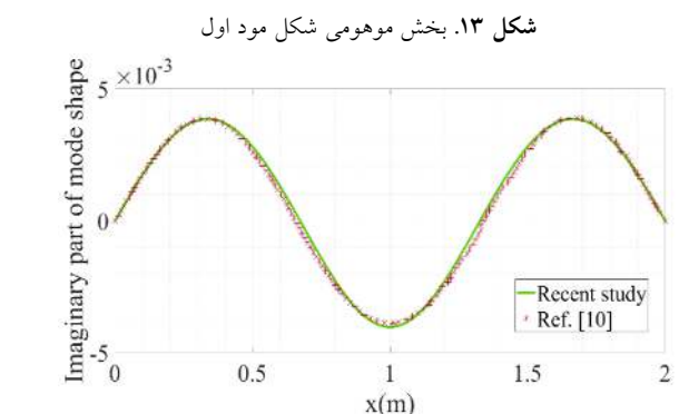
Fig. 13. Imaginary part of the first mode shape
