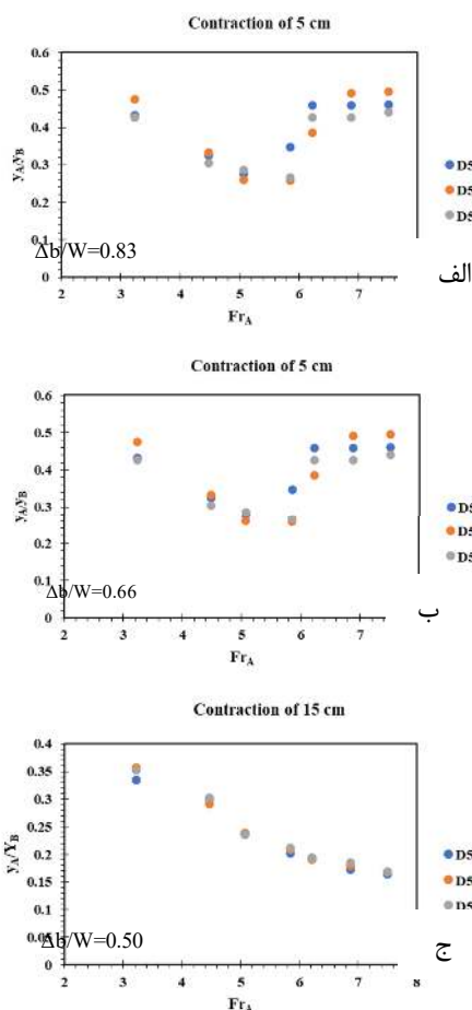
Fig. 10. Variation of conjugated depth versus vena contracta Froude number
