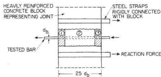
Fig. 19. Elingausen schematic test setup [1]
