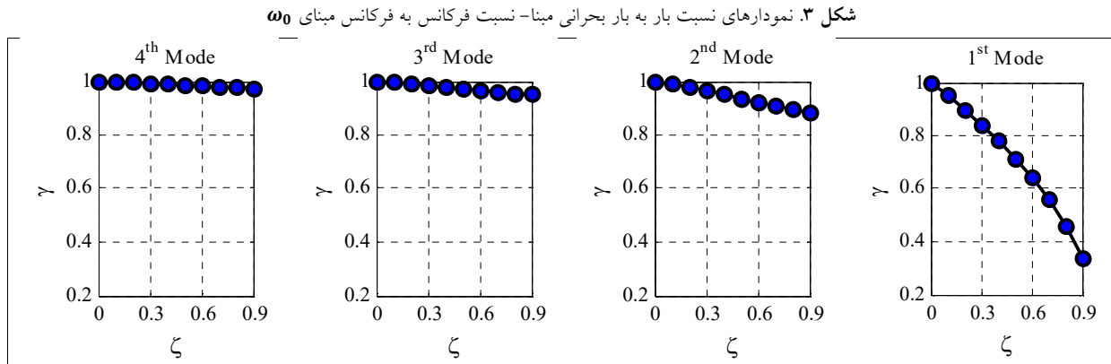
Fig. 3. Graphs of the ratio of load to basic critical load- the ratio of frequency to basic frequency \omega_0
