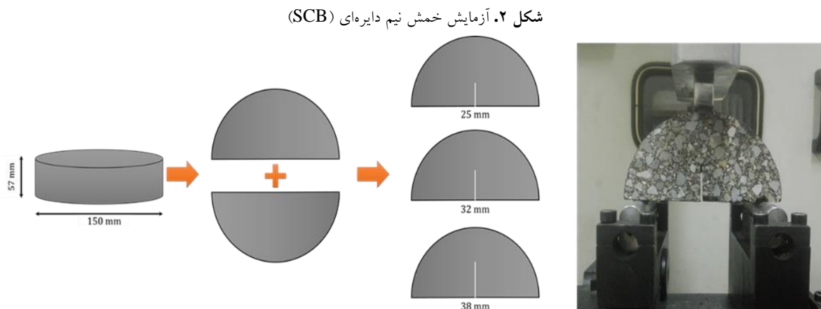
Fig. 2. Semi-circular bending (SCB) test
