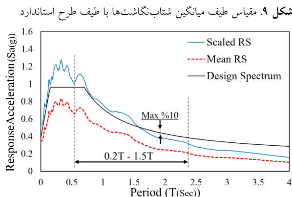
Fig. 9. Scaled mean spectrum to design spectrum
