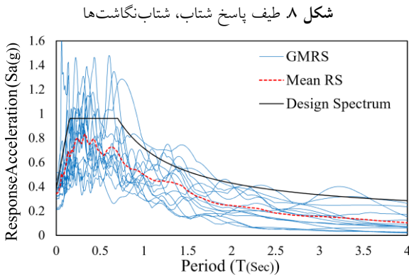
Fig. 8. Acceleration response spectrum of records
