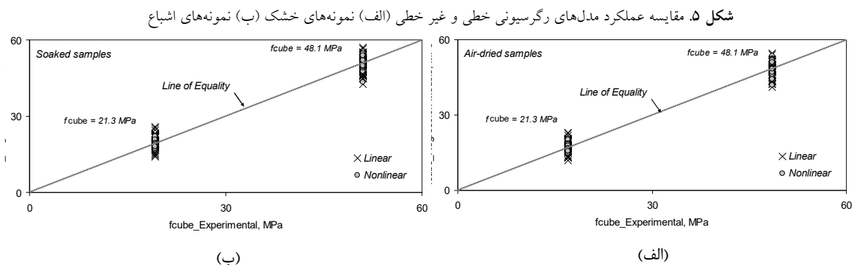
Fig. 5. Comparison of the performance of linear and nonlinear regression models (a) Air-dried samples (b) Soaked samples
