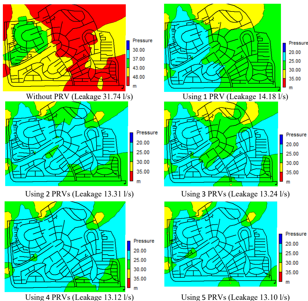
Fig. 5. Pressure distribute at 3:00am in no-valve mode and 1 to 5 installed PRV
