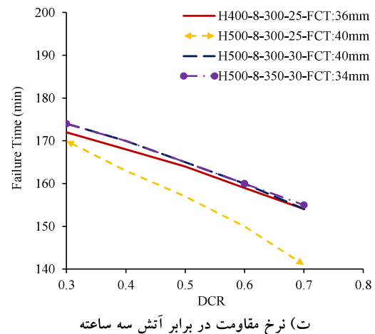
Fig. 5. Column failure time versus DCR
