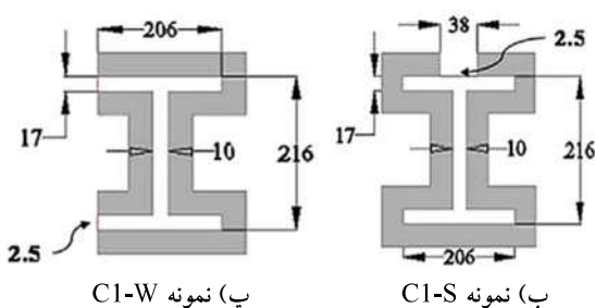
Fig. 1. Geometrical details of specimens
