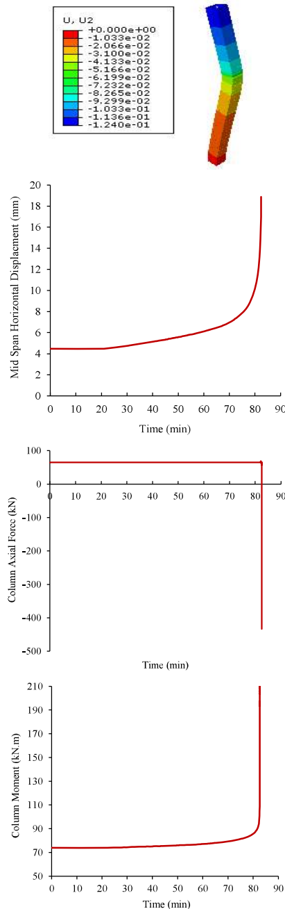
Fig. 3. Deformed shape, mid-span horizontal displacement, axial force, and bending moment of column Box200x15 with FCT (12mm) and DCR (70%)
