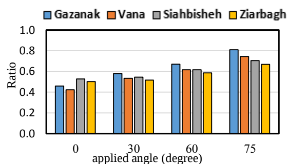
Fig. 7. Ratio of abutment unseating under different angles to that with the application angle of 90 degrees under the Northridge earthquake.
