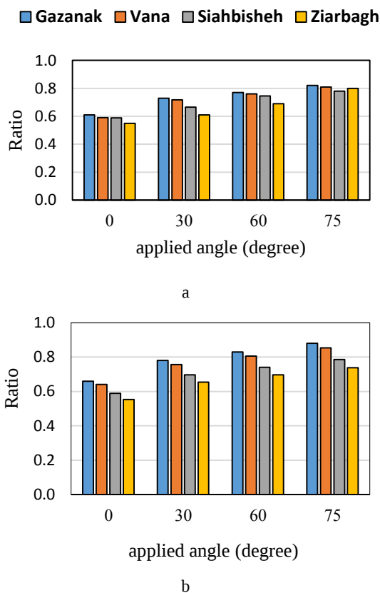
Fig. 6. (a) Ratio of curvature at arch midspan under the 90-degree incidence angle under the Manjil earthquake; (b) Ratio of curvature ductility demand at arch midspan under different incidence angles to the value corresponding to the 90-degree angle under the Kocaeli earthquake
