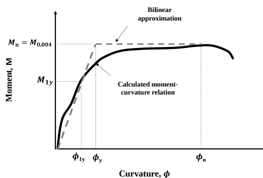
Fig. 4. Moment-curvature diagram and bilinear approximation
