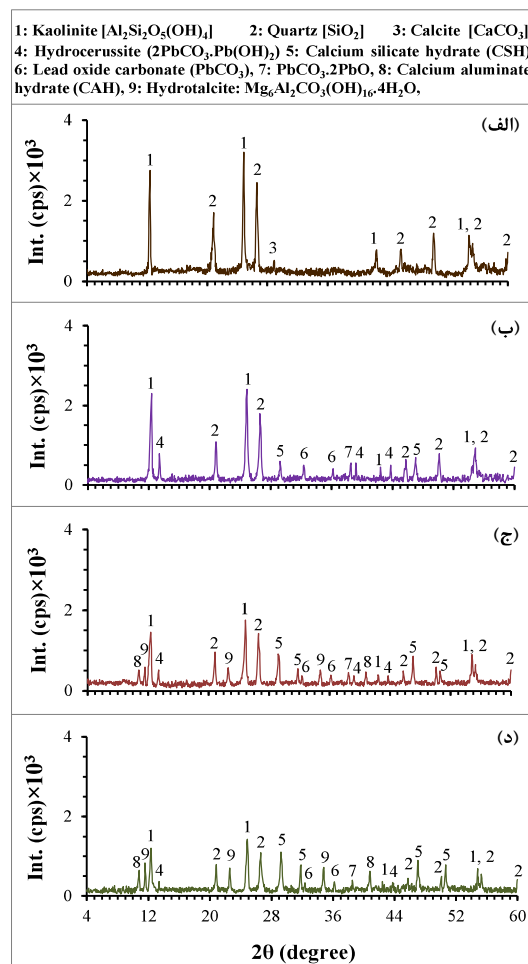
Fig. 6. XRD patterns: (a) Natural soil, (b) S/S sample with cement, (c) S/S sample with SGZ, (d) S/S sample with SGZP
