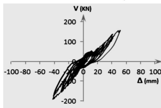
Fig. 10. Hysteresis curve of MO2
