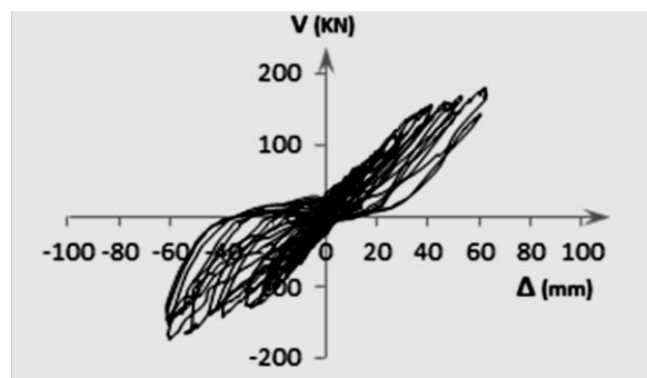
Fig. 12. Hysteresis curve of SPC2
