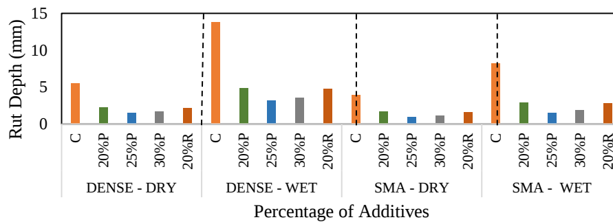
Fig. 4. Wheel Track Testing Results (7500 Cycles and 50 ° C)
