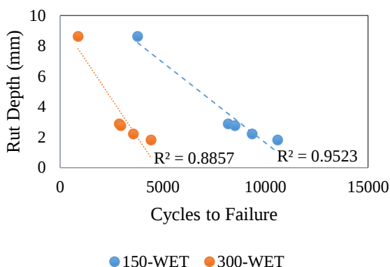
Fig. 7. Correlation between RLA and HWT test
