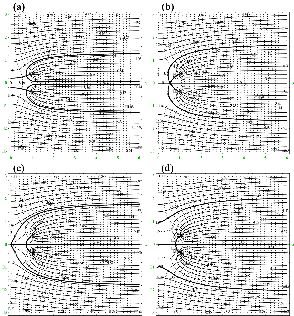
Fig. 3. The flow field for double-well system, configuration (I) for d_D=0.4 : (a): Q_D=0.200 , (b): Q_D=Q_{C2}=0.271 , (c): Q_D=Q_{C1}=0.290 , (d): Q_D=0.333 (Solid lines display Position of capture zone, Dashed lines display Equipotential lines, and Thin lines display Stream lines)
