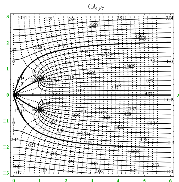
Fig. 4. The flow field for double-well system, configuration (II) for d_D = 0.578, Q_D = Q_{C1} = Q_{C2} = 0.333 (Solid lines display Position of capture zone, Dashed lines display Equipotential lines, and Thin lines display Stream lines)
