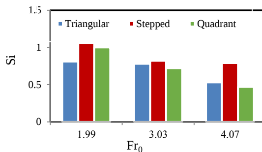
Fig. 6. Values of scour index for W/D_e = 4.23
