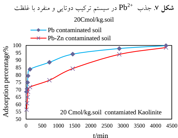
Fig. 7. Adsorption of Pb^{2+} in single and binary-component systems with 20 Cmol kg^{-1} concentration.
