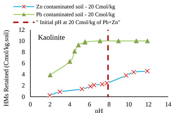
Fig. 2. The adsorption rate of Pb^{2+} and Zn^{2+} in the pH ranged from 2 to 12 for concentration 20 Cmol kg -1 in the binary-component system.
