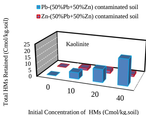
Fig. 4. Changes in Pb^{2+} and Zn^{2+} absorption rates in the binary-component systems with various concentrations.
