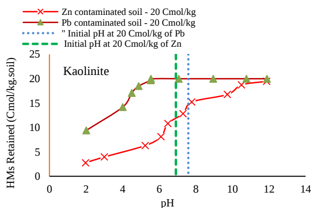
Fig. 1. The adsorption rate of Pb^{2+} and Zn^{2+} in pH range of 2 to 12 for concentration of 20 Cmol kg -1 in a single-component system.
