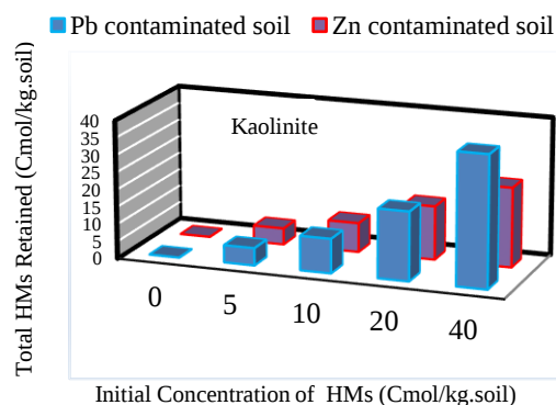
Fig. 3. Changes in Pb^{2+} and Zn^{2+} absorption rates in the single-component systems with various concentrations.
