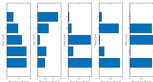
Fig. 27. Axial forces at bracing frame floors for RMS (20%, 15%).
